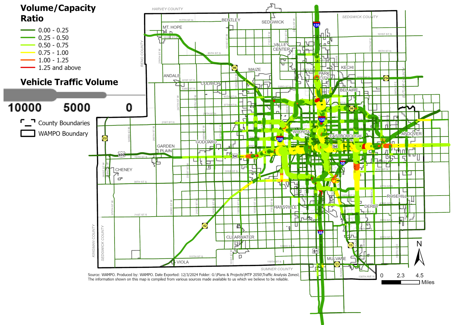
Map E.4: WAMPO TDM 2022 Base Scenario AM-Peak Traffic Volumes and Congestion Levels
