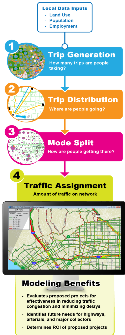
Figure E.1: Travel Demand Modeling Process
