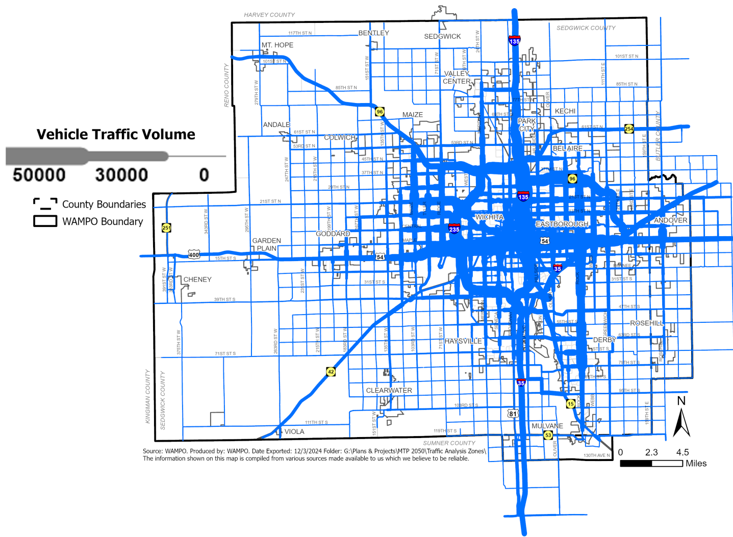
Map E.3: WAMPO TDM 2050 Build Scenario Daily Traffic Volumes
