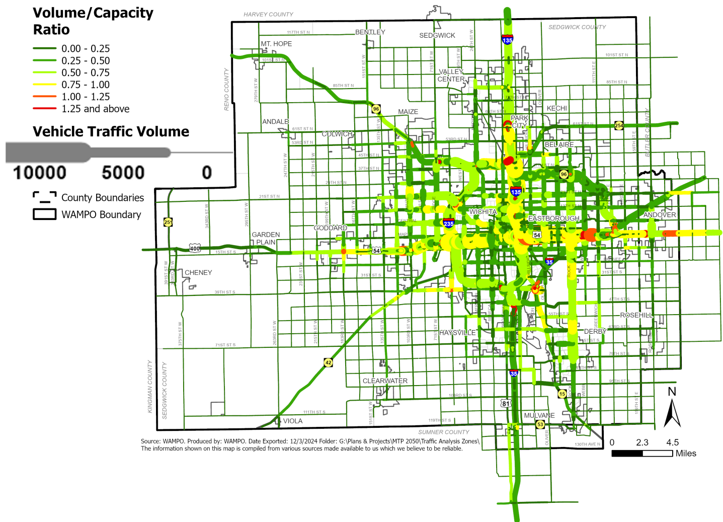
Map E.5: WAMPO TDM 2050 Build Scenario AM-Peak Traffic Volumes and Congestion Levels
