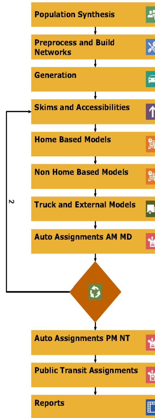
Figure E.2: WAMPO Travel Demand Model Structure
